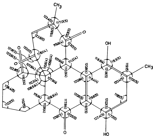
Fig. 3. Bond angles ( \phi/^\circ ) of 7Bd.
